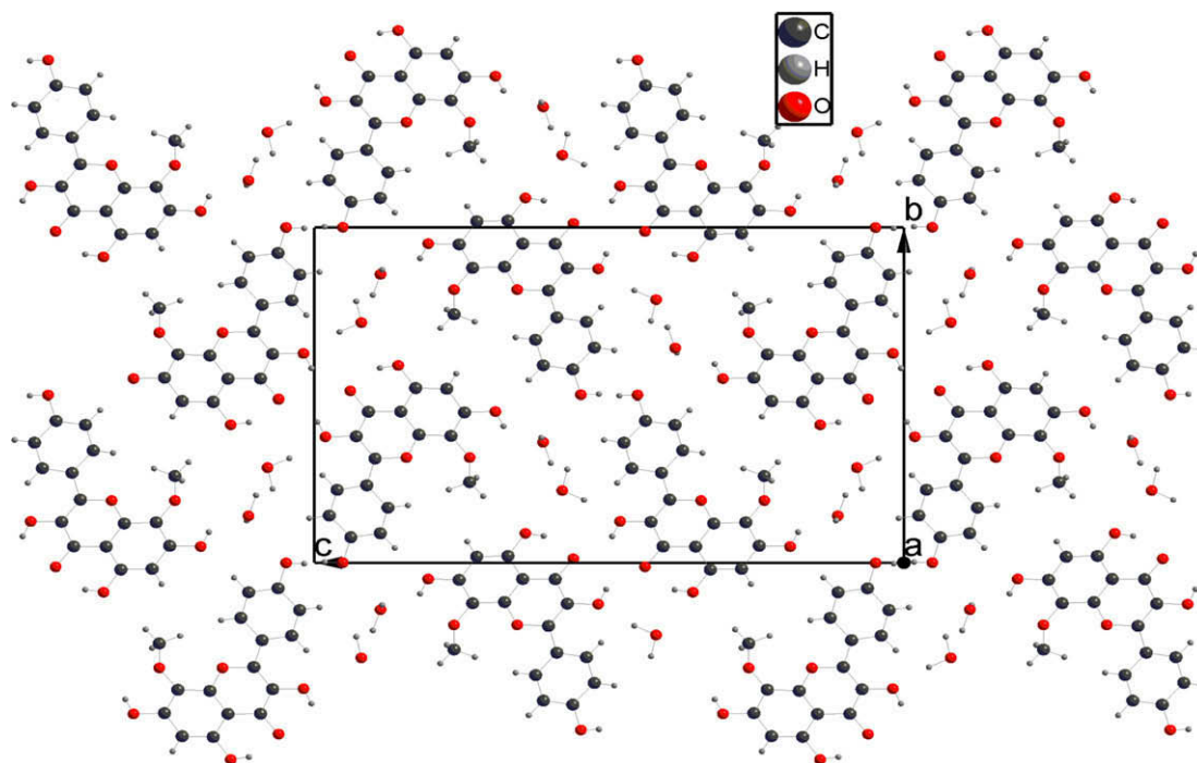
Figure 3 A projection, along [1 0 0], of the crystal structure of flavonoid (2).
