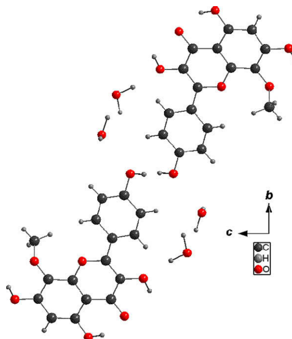
Figure 2 Dimer [(C_{16}H_{12}O_7) \cdot 2H_2O]_2 in the crystal of flavonoid ( 2 ).
