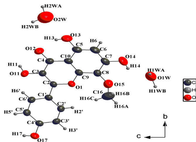
Figure 1 Perspective view, (Diamond Brandenburg, 1999), of the molecule of flavonoid ( 2 ). Thermal ellipsoids drawn at 50% probability levels.
